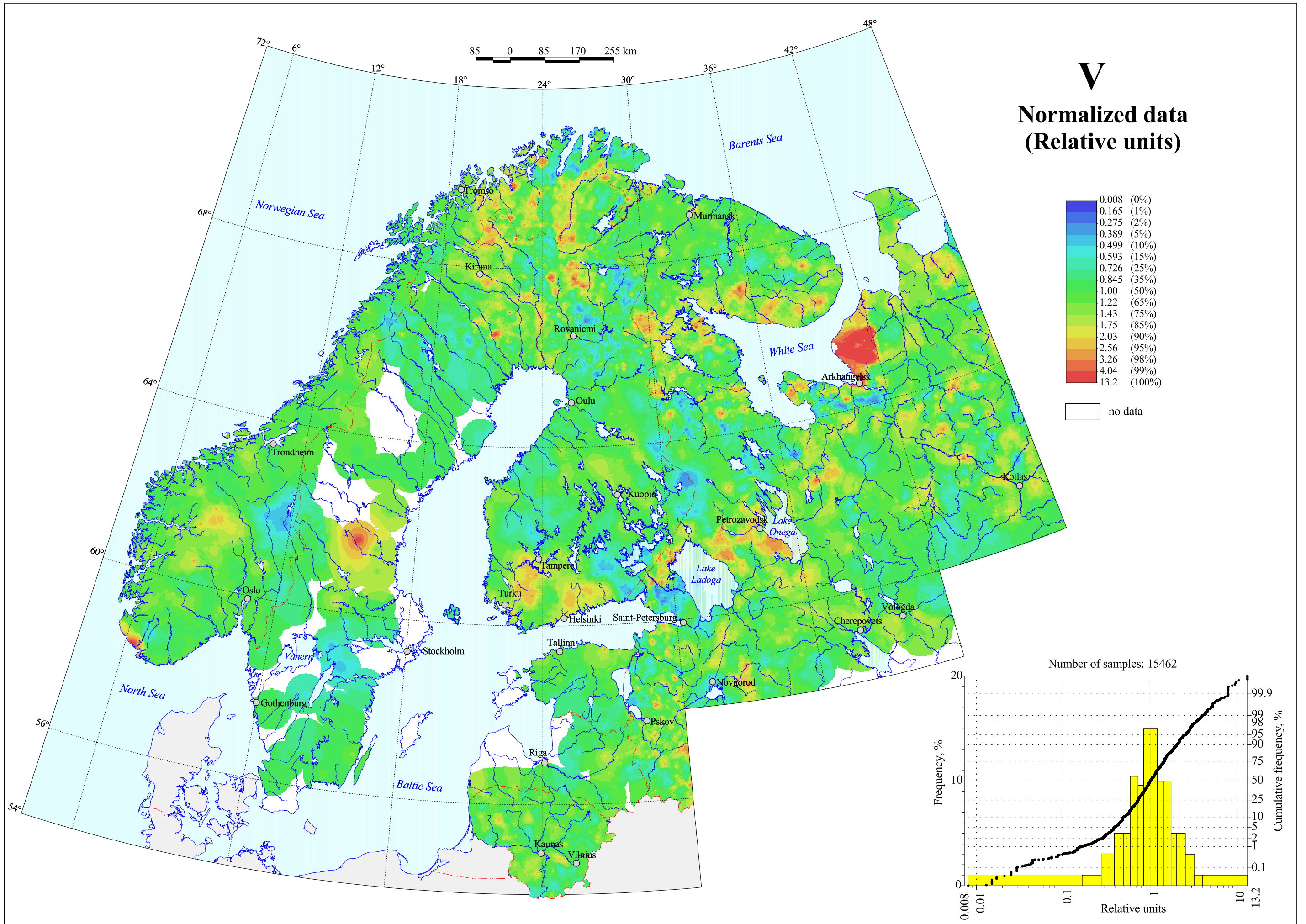
Vanadium in Stream Sediment
